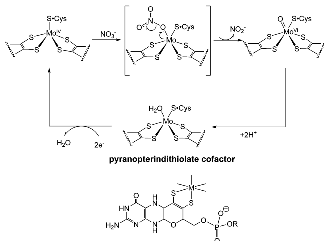
Figure 1. Schematic depictions of the reduced and oxidized sites of dissimilatory nitrate reductase ( Desulfovibrio desulfuricans ) and the proposed reaction pathway. Also shown is the pyranopterindithiolate cofactor (R absent or a nucleotide).
